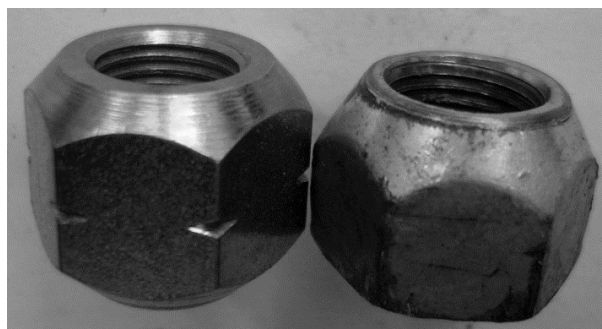
The wheel nut on the left has the correct taper for RM wheels.
