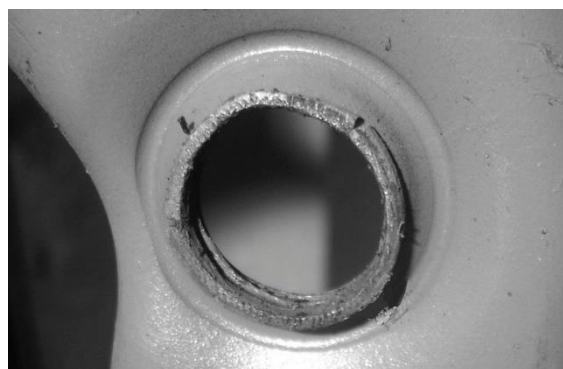
This wheel stud hole has been forcibly expanded by a nut with too steep a taper angle, as shown on the right below.
