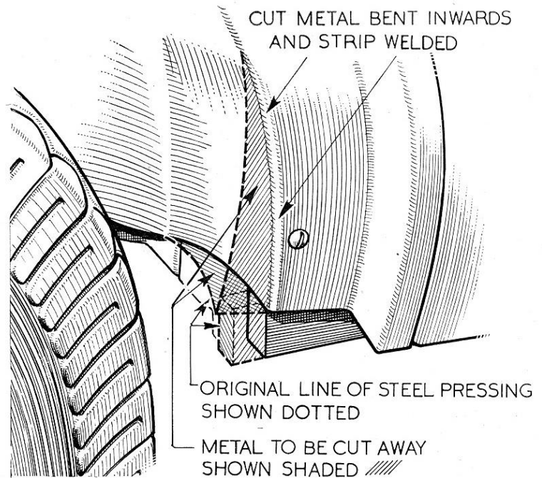
This sketch shows the positions of sawcuts and weld in order to give extra clearance for the snow chain.
